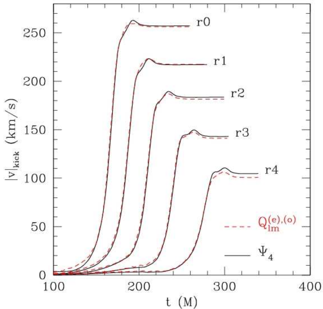
Fig. 1.— Net recoil speed as a function of time, for various initial separations of two spinning black holes. These realizations are from the group at the Albert Einstein Institute in Potsdam, Germany. From http://numrel.aei.mpg.de/Images/vkick-vs.time.jpg
